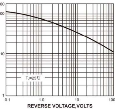
FIG. 5-TYPICAL JUNCTION CAPACITANCE
