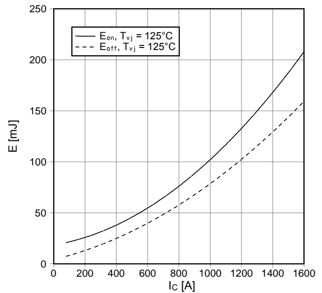
Schaltverluste IGBT-Wechselr. (typisch) switching losses IGBT-inverter (typical) E_{on} = f(I_c) , E_{off} = f(I_c) V_{GE} = \pm 15\text{ V} , R_{Gon} = 1,3\ \Omega , R_{Goff} = 1,3\ \Omega , V_{CE} = 600\text{ V}
