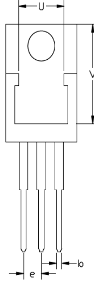
Btm View
