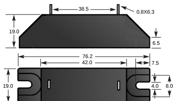
Outline Drawings : mm
