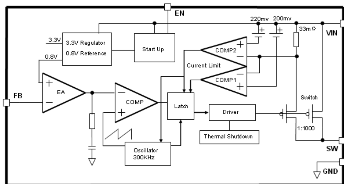
Figure3. Function Block Diagram of XL4003
