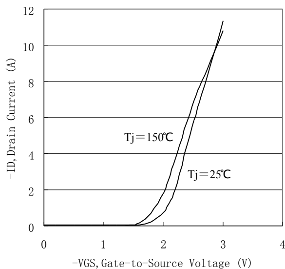
Figure 2. Transfer Characteristics
