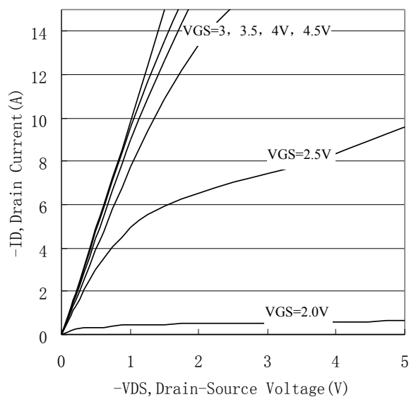
Figure 1. Output Characteristics
