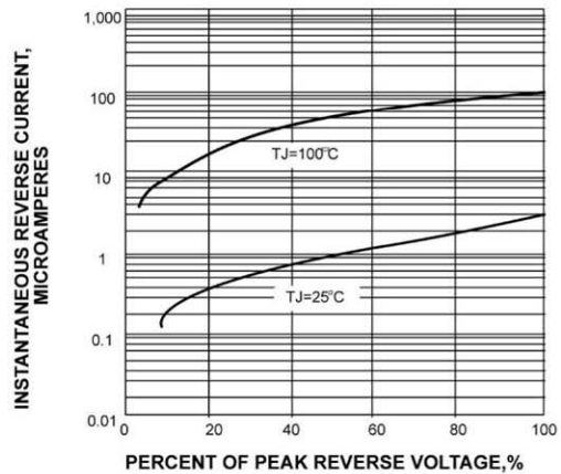
FIG. 4-TYPICAL REVERSE CHARACTERISTICS
