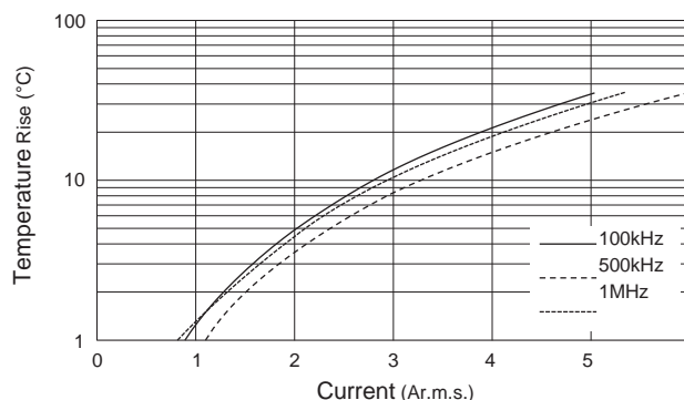
Ripple Current
