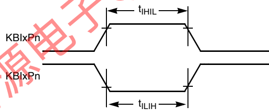
Figure 18. KBlxPn Timing
