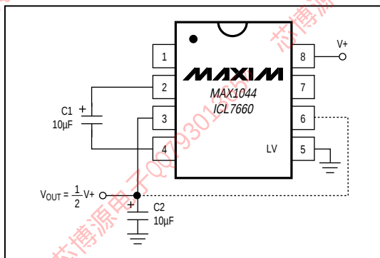
Figure 10. Voltage Divider
