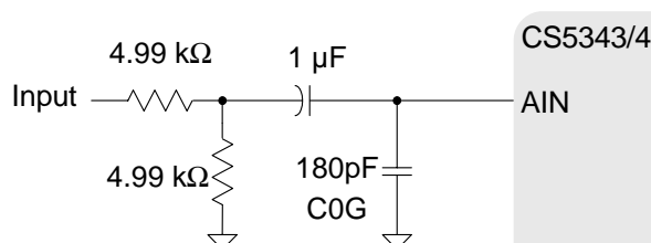
Figure 7. CS5343/4 Example Analog Input Network
