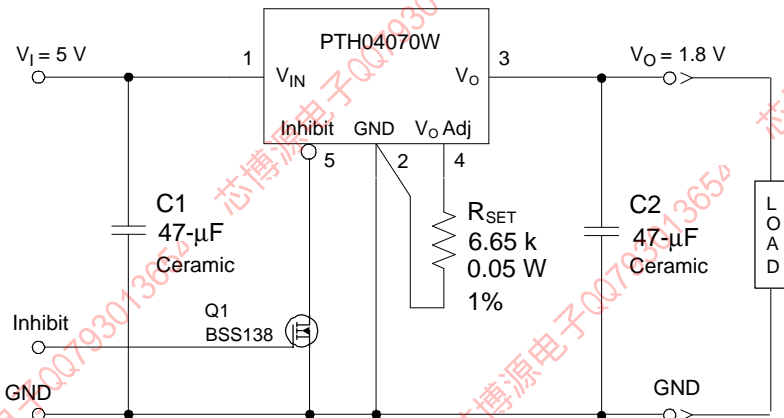
Figure 11. On/Off Inhibit Control Circuit
