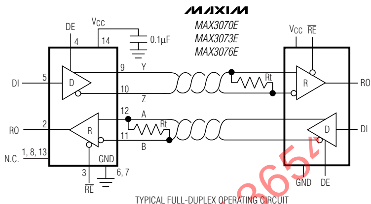
TYPICAL FULL-DUPLEX OPERATING CIRCUIT
