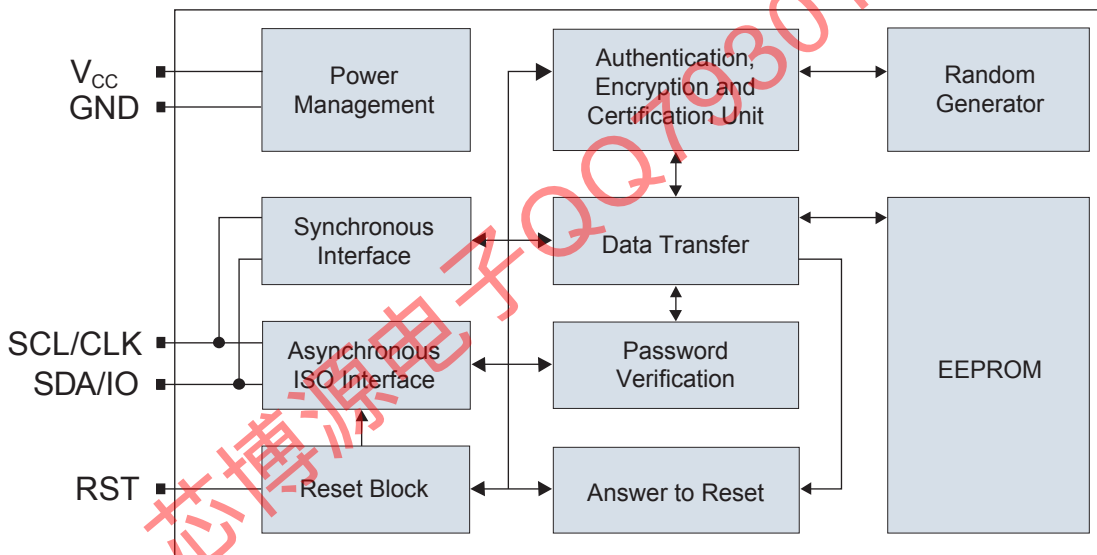
Figure 2. Block Diagram
