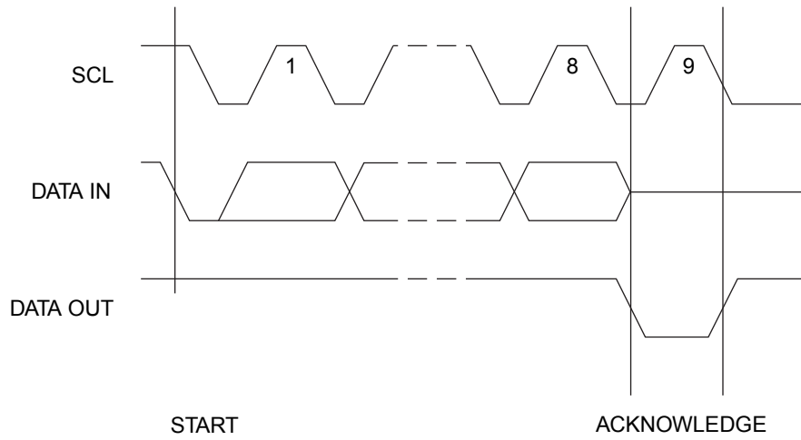
Figure 8. Output Acknowledge
