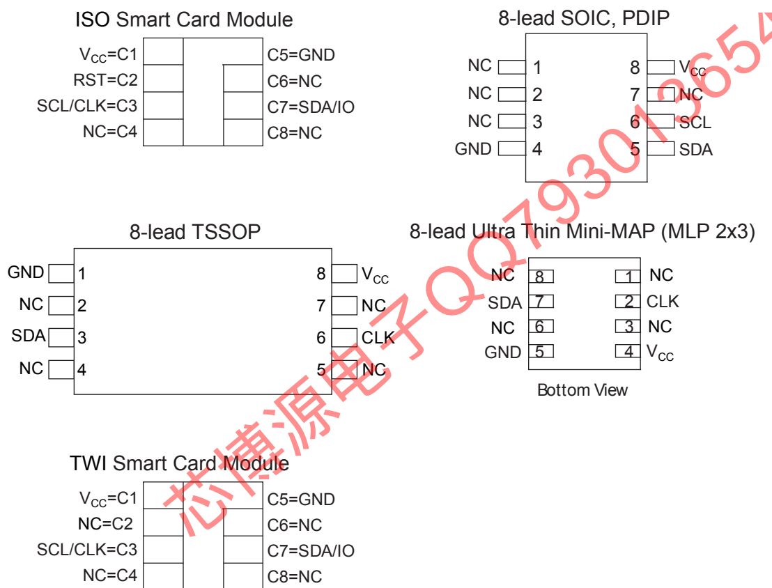
Figure 1. Pin Configuration
