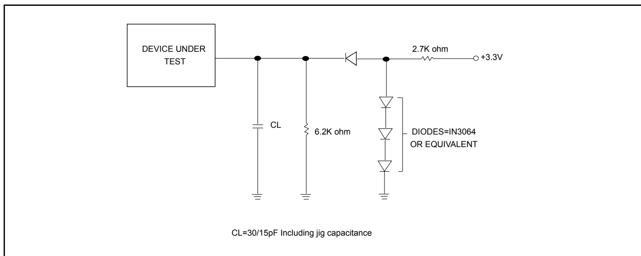
Figure 41. Output Loading
