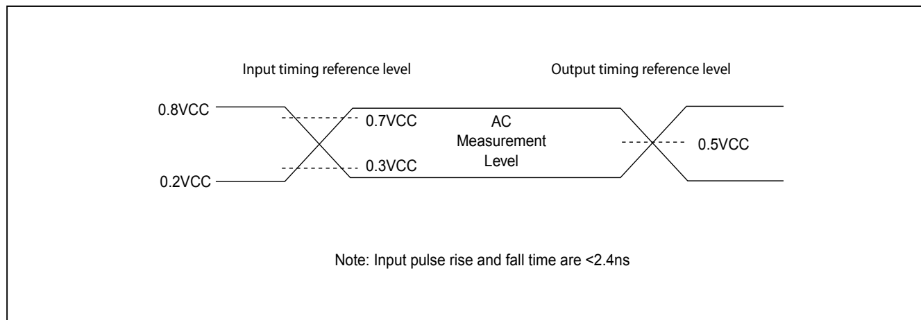
Figure 40. Data Input Test Waveforms and Measurement Level
