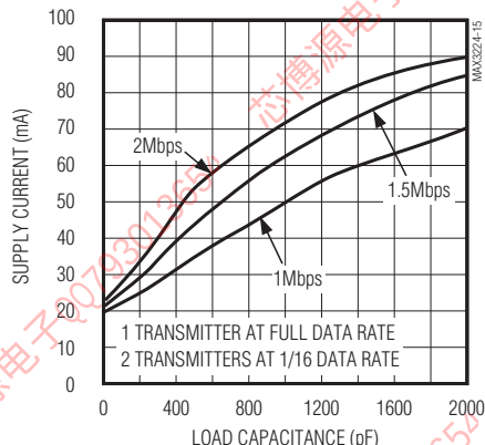
MAX3245 OPERATING SUPPLY CURRENT vs. LOAD CAPACITANCE
