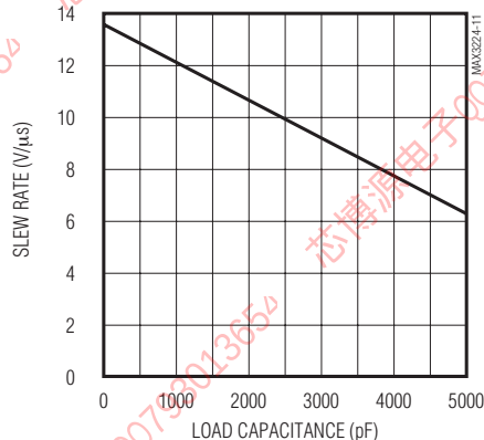
MAX3244 SLEW RATE vs. LOAD CAPACITANCE
