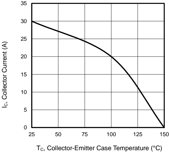
Figure 14 Current Derating
