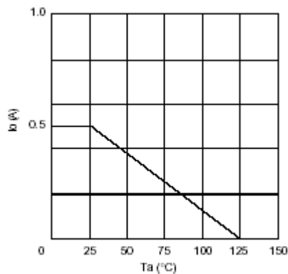
Fig.4 Derating curve
