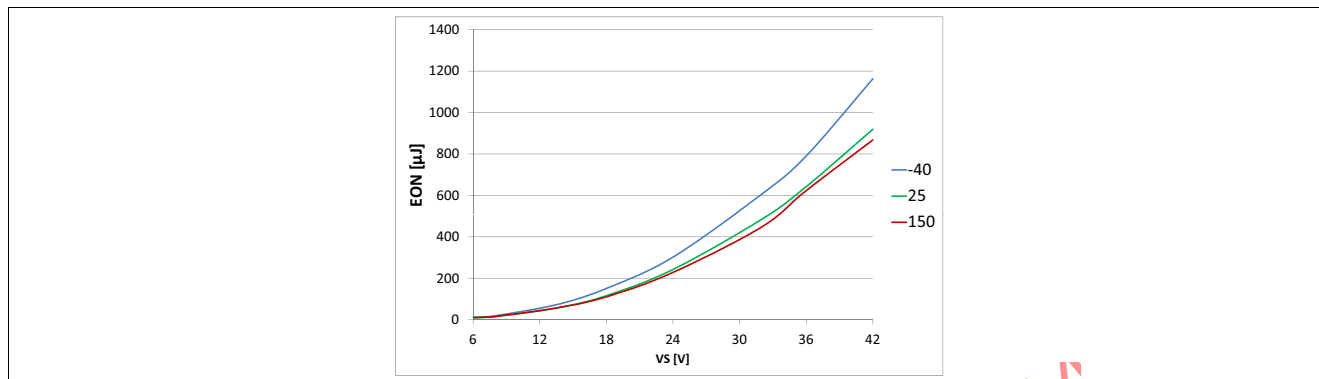
Figure 40 Switch ON Energy E_{ON} = f(T_J; V_{GS}), R_L = 12 \Omega
