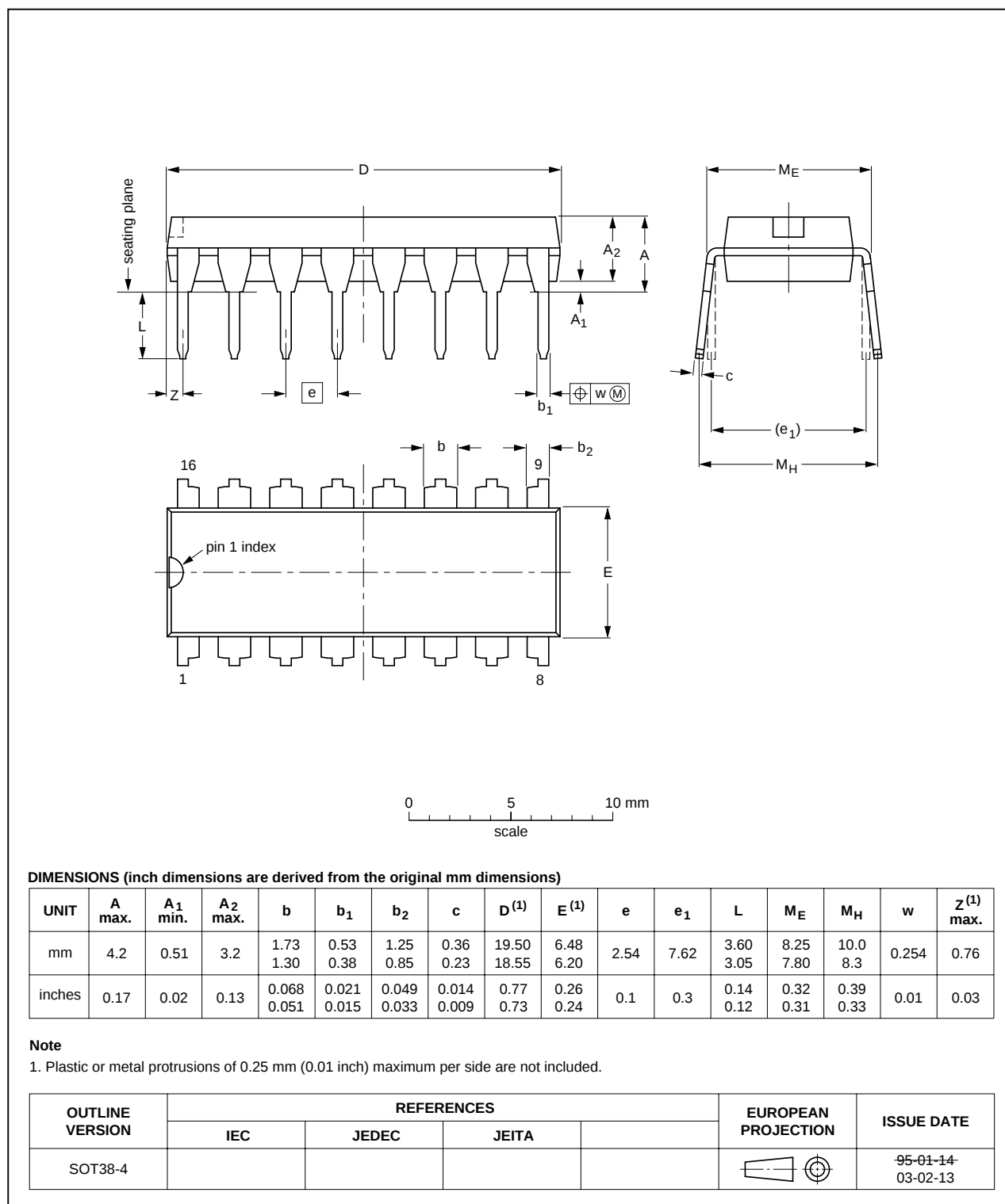
Fig 18. Package outline SOT38-4 (DIP16)
