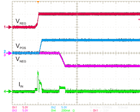
Figure 40. Inrush Current — Sequential
