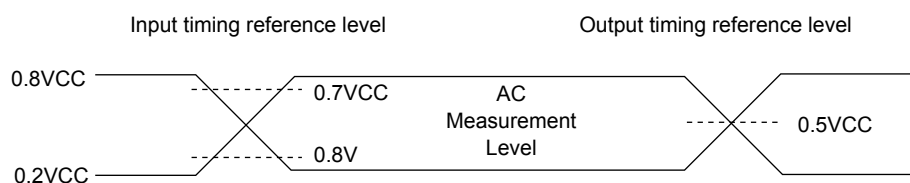
Figure 72. INPUT TEST WAVEFORMS AND MEASUREMENT LEVEL
