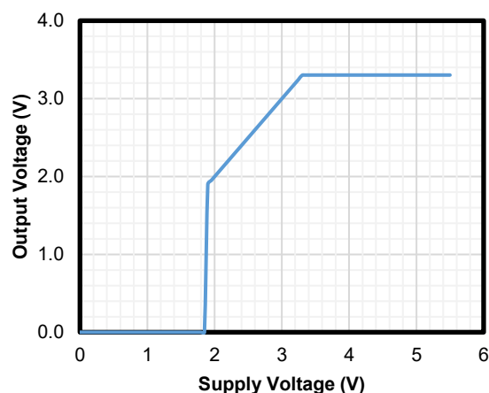
Figure 6. Output Voltage vs Supply Voltage
