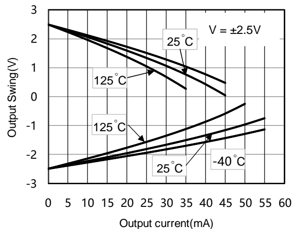
OUTPUT SWING vs LOAD CURRENT
