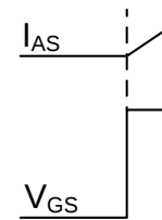
Fig.8 EAS Waveform
