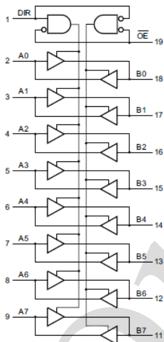
Figure 1. Logic symbol
