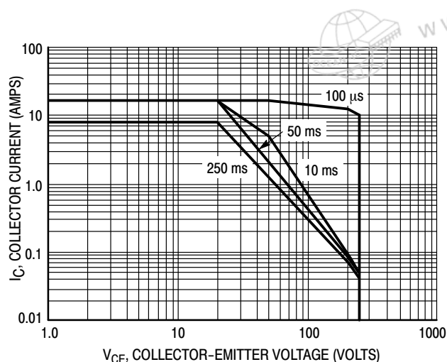
Figure 2. MJE15032 & MJE15033 Safe Operating Area
