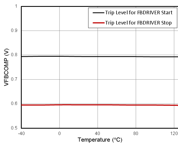
Fig14. Threshold for FB Burst Mode vs. Temperature
