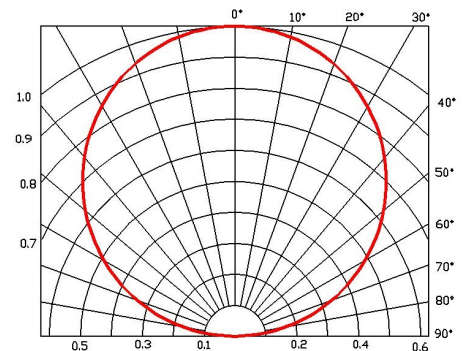
Radiation angle
