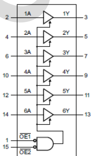
Figure 3. Functional diagram
