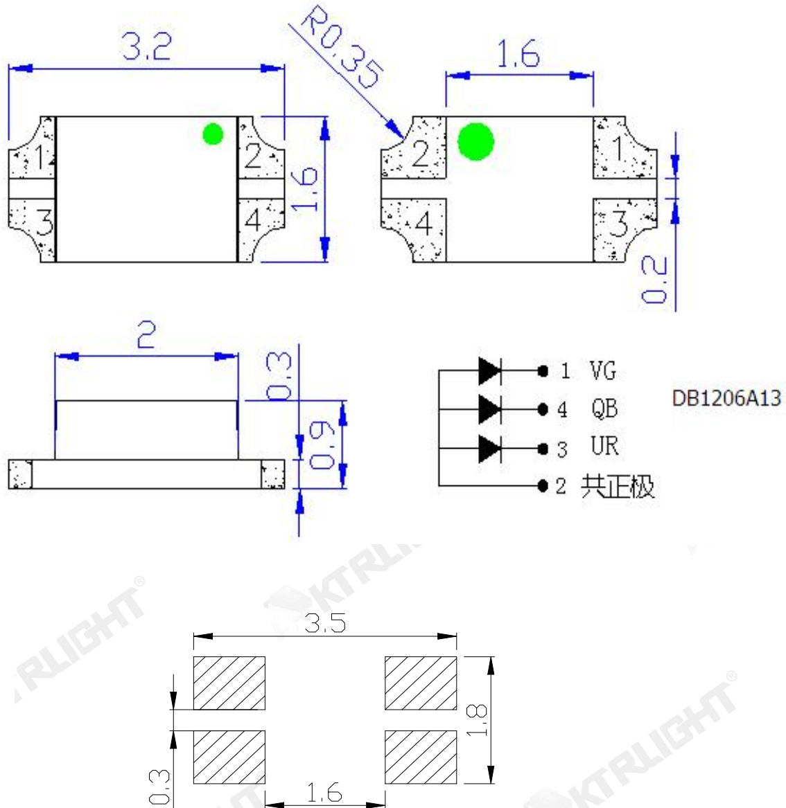
推荐焊盘尺寸 Recommended Soldering Pattern
