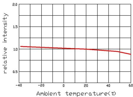
Relative light intensity vs ambient temperature
