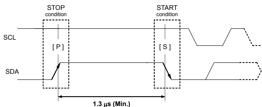
Figure 8-26. I2C bus START STOP condition
