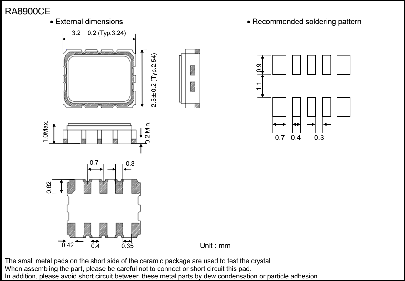
Figure 9-1. RA8900CE package
