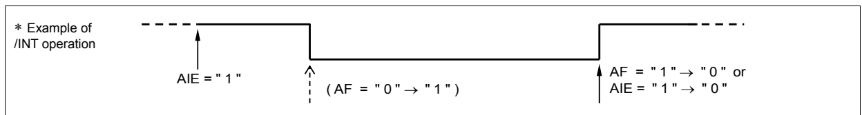
Figure 8-10. Alarm Interrupt
