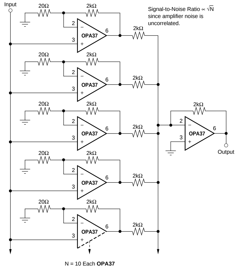
FIGURE 16. Ultra-Low Noise "N"-Stage Parallel Amplifier.
