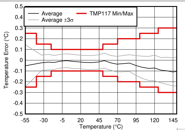
图 6-2. DRV Package Temperature Error vs Temperature
