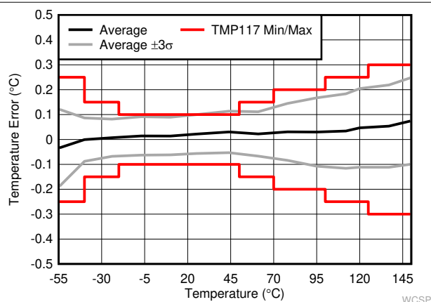
图 6-3. YBG Package Temperature Error vs Temperature
