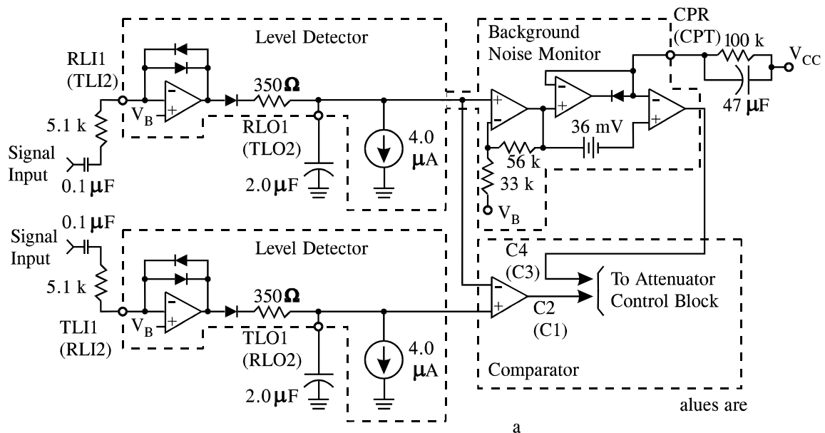
Figure 2. Level Detectors
