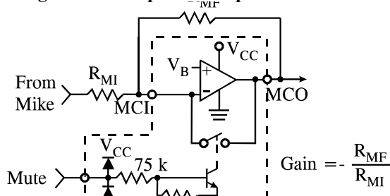
Figure 5. Microphone Amplifier and MUTE
