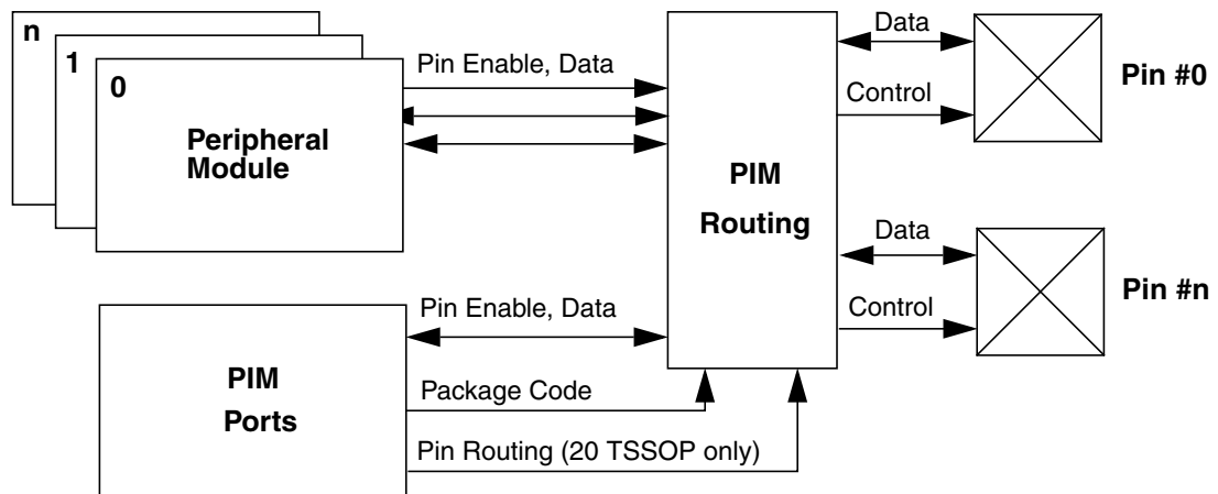
Figure 2-1. Block Diagram
