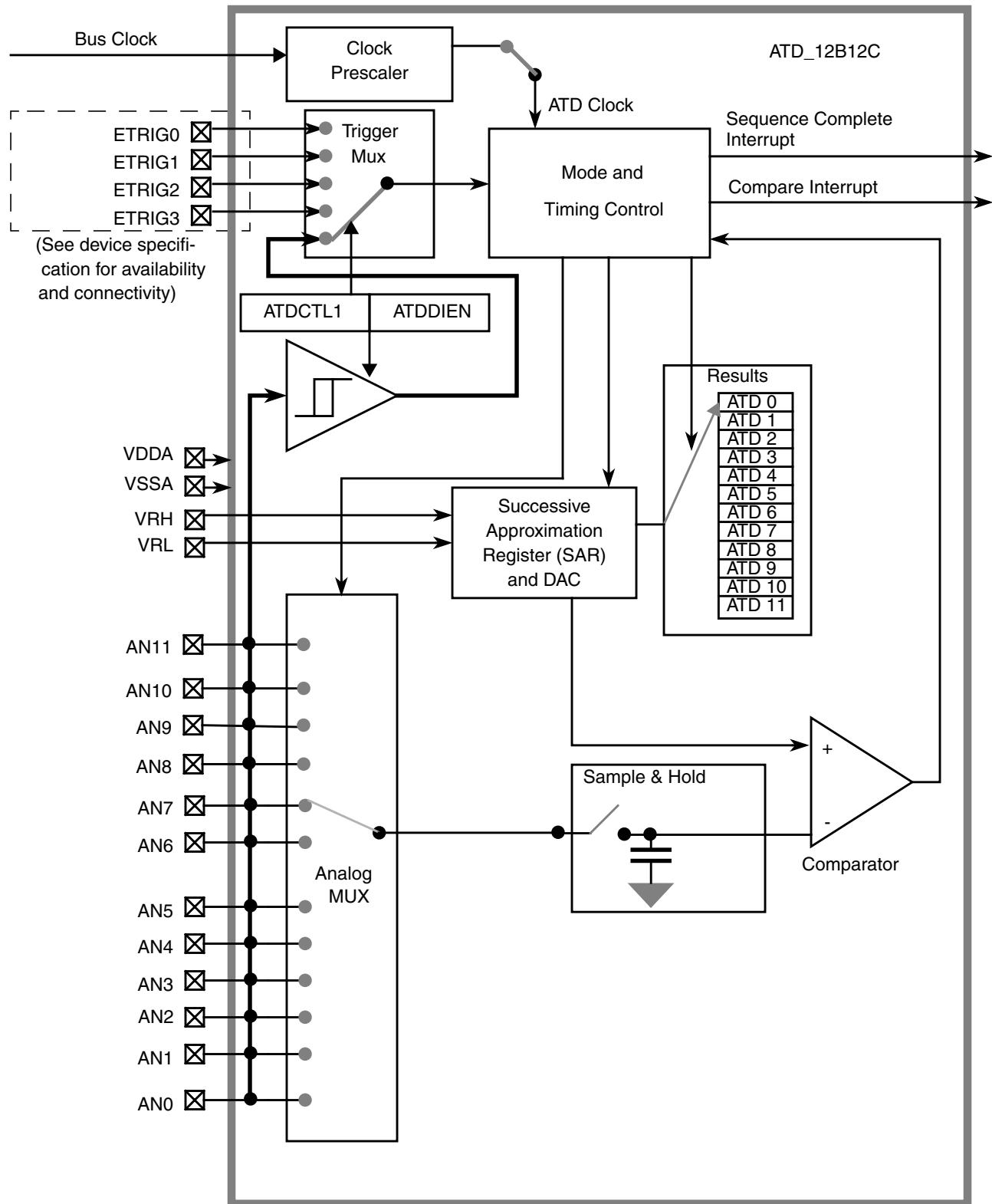
Figure 12-1. ADC10B12C Block Diagram
