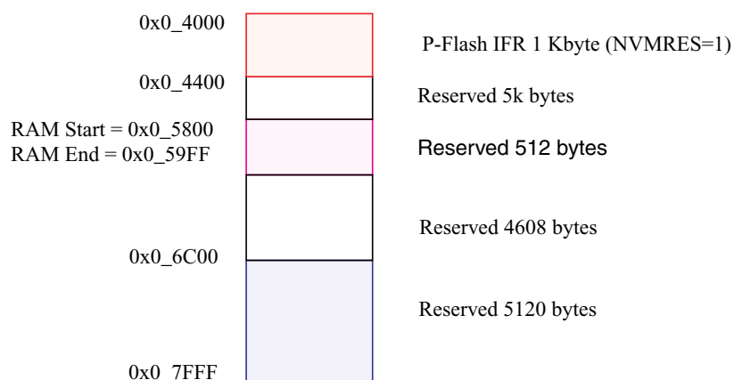
Figure 23-3. Memory Controller Resource Memory Map (NVMRES=1)
