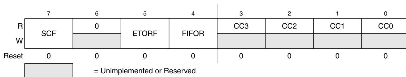
Figure 11-9. ATD Status Register 0 (ATDSTAT0)
