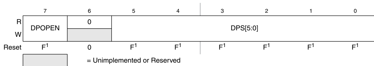
Figure 23-15. EEPROM Protection Register (EPROT)
