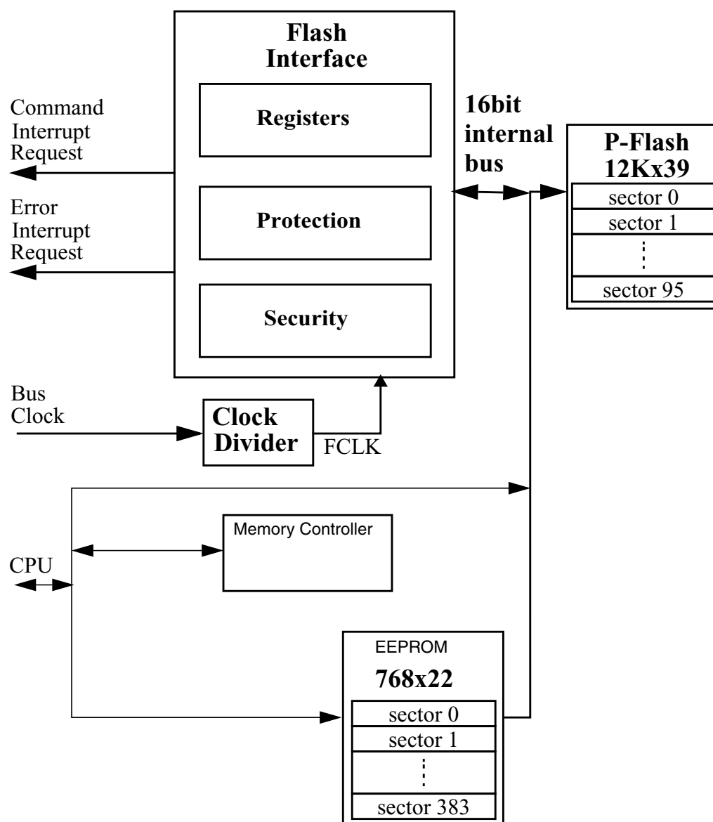
Figure 23-1. FTMRG48K1 Block Diagram
