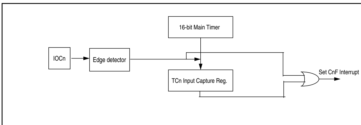
Figure 20-3. Interrupt Flag Setting
