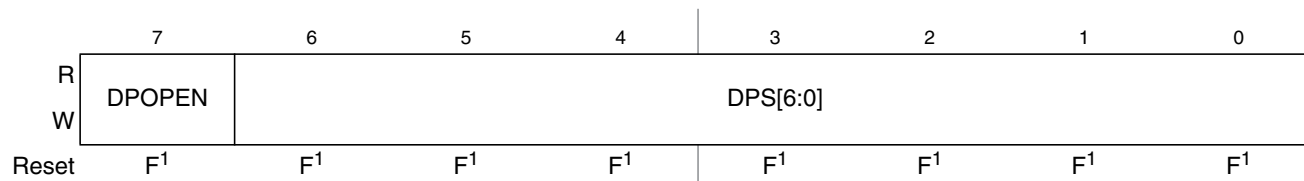
Figure 26-15. EEPROM Protection Register (DFPROT)
