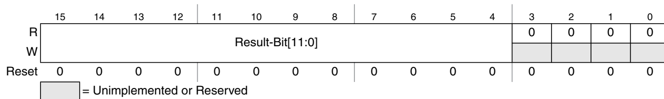
Figure 13-14. Left justified ATD conversion result register (ATDDRn)
