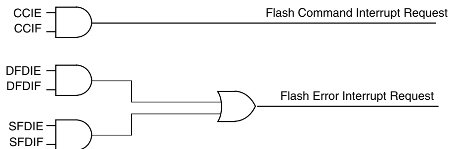
Figure 23-27. Flash Module Interrupts Implementation
