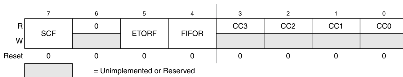
Figure 13-9. ATD Status Register 0 (ATDSTAT0)
