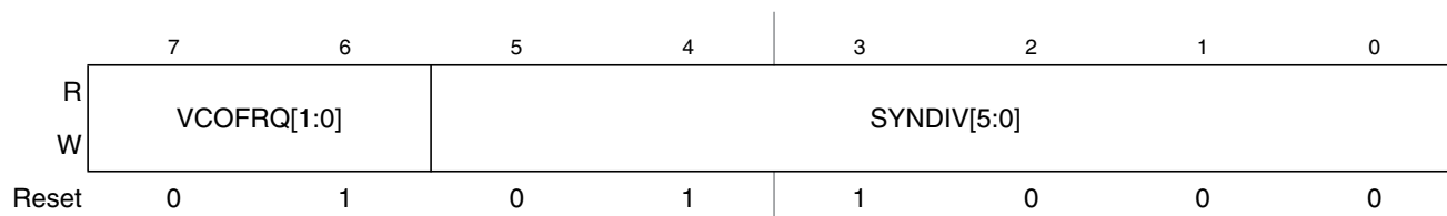
Figure 10-4. S12CPMU Synthesizer Register (CPMUSYNR)
