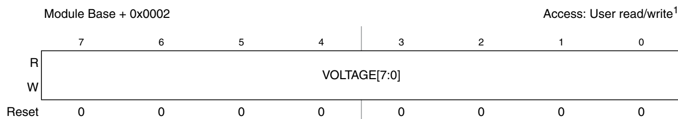
Figure 15-4. Analog Output Voltage Level Register (DACVOL)
