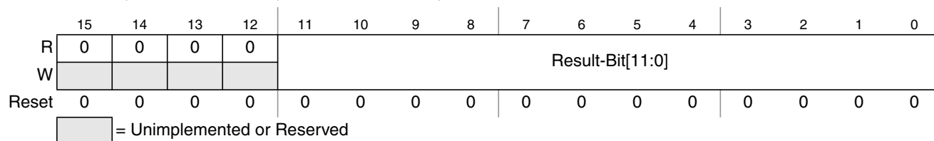
Figure 12-15. Right justified ATD conversion result register (ATDDR n )
