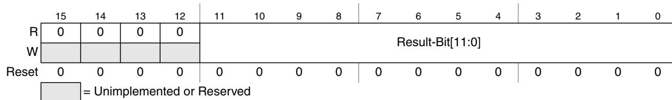
Figure 11-15. Right justified ATD conversion result register (ATDDR n )
