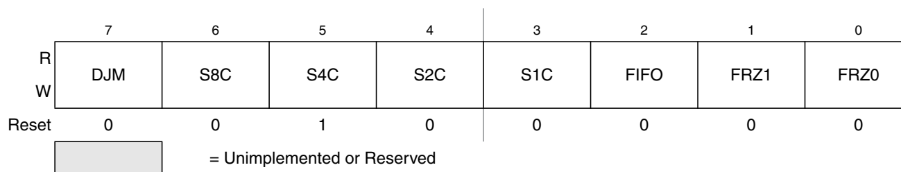
Figure 11-6. ATD Control Register 3 (ATDCTL3)
