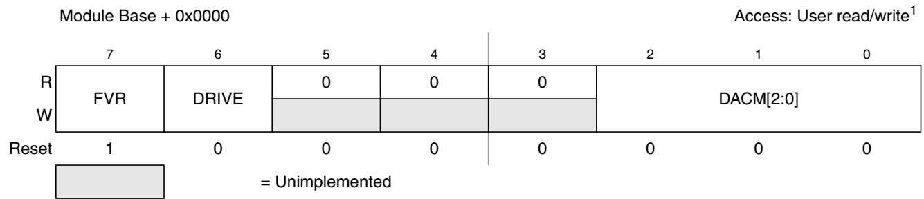
Figure 15-3. Control Register (DACCTL)
