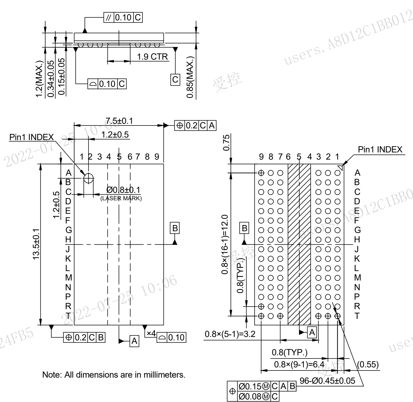
Figure 4. Package Dimensions
