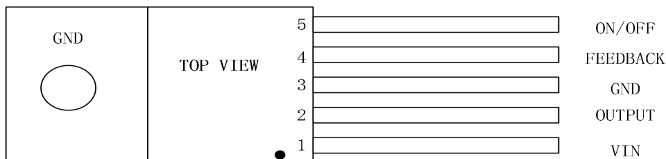
TO220-5
