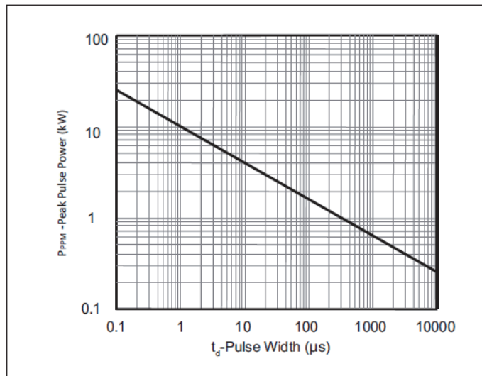
Figure 2. Peak Pulse Power Rang Curve
