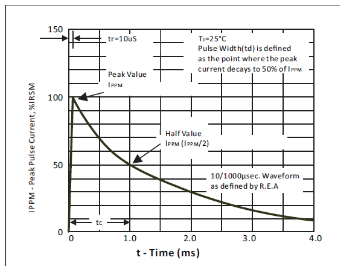
Figure 4. Pulse Waveform
