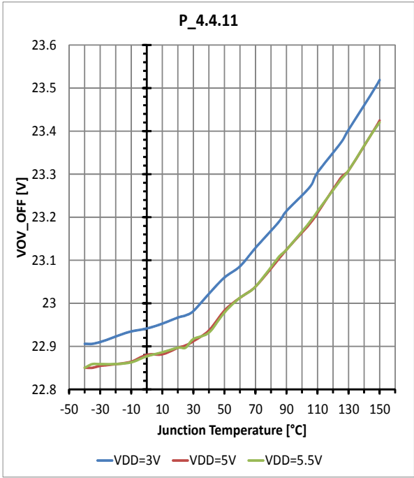
Overvoltage switch OFF voltage threshold
