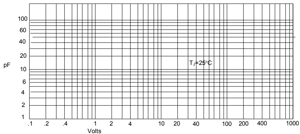
Figure 3 Junction Capacitance
