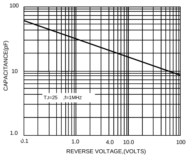
FIG.3-TYPICAL JUNCTION CAPACITANCE
