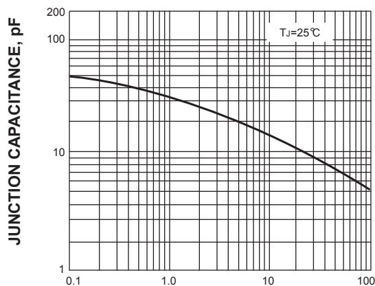
FIG. 5-TYPICAL JUNCTION CAPACITANCE
