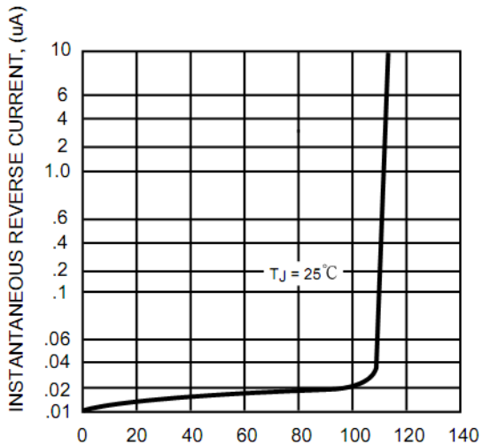
TYPICAL REVERSE CHARACTERISTICS PERCENT OF RATED PEAK REVERSE VOLTAGE, (%)
