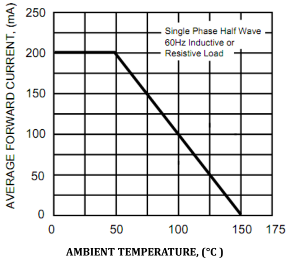
TYPICAL FORWARD CURRENT DERATING CURVE
