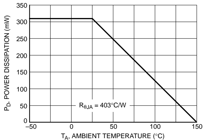
FIG.1 Derating Curve
