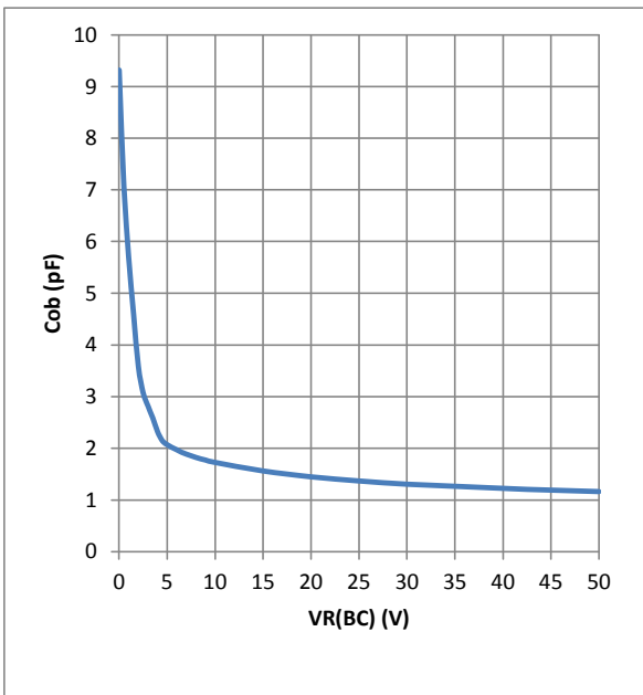
FIG.4 Output Capacitance
