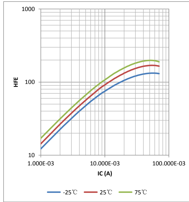
FIG.3 DC Current Gain
