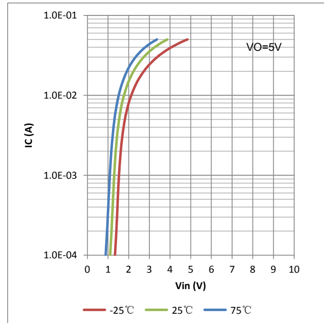
FIG.5 Output Current vs. Input Voltage
