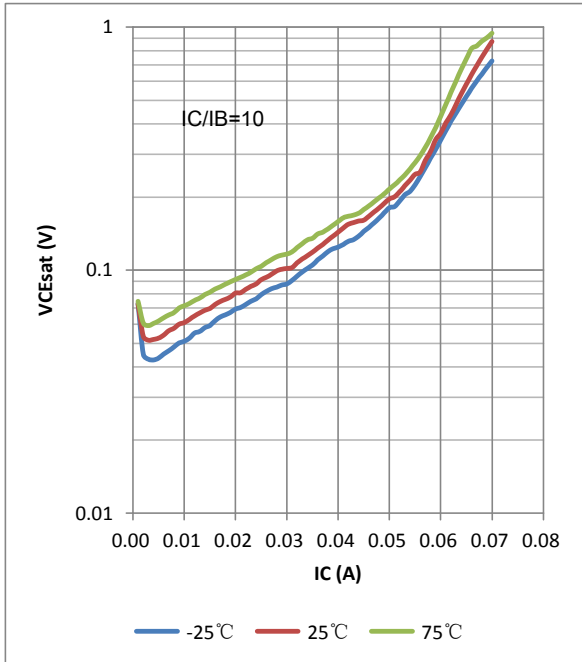
FIG.2 V_{CE(sat)} vs. I_C
