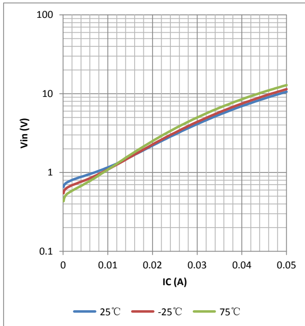
FIG.6 Input Voltage vs. Output Current
