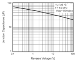
Figure 5. Typical Junction Capacitance Per Leg
