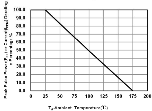
FIG.2-Pulse Derating Curve
