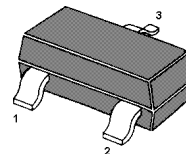
1.Reference 2.Cathode 3. Anode SOT-23 Plastic Package
