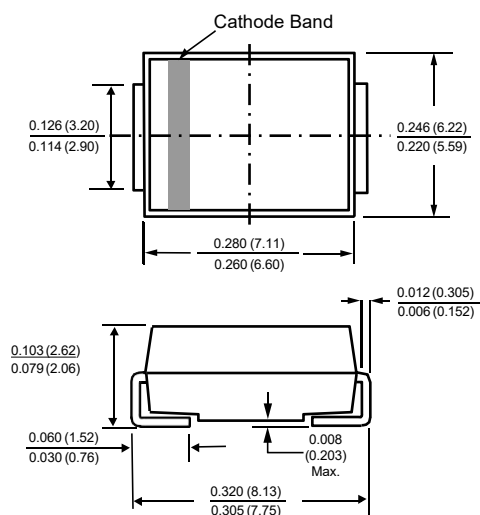
SMC (DO-214AB)
